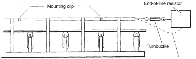
Figure 4A Side view
