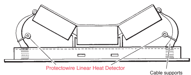
Figure 3B End view
