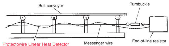
Figure 3A side view
