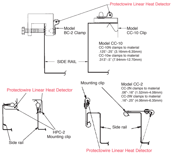
Figure 10B Typical Cable Tray Mountings
