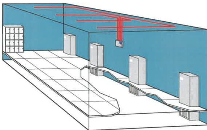
Secondary Detection Example (All sampling points located in the position of 'point type' smoke detectors)
