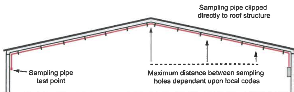
Secondary Detection Example (All sampling points located in the position of 'point type' smoke detectors)
