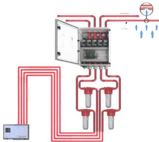
Protec Cirrus Pro detector with typical pipe purging unit connection
