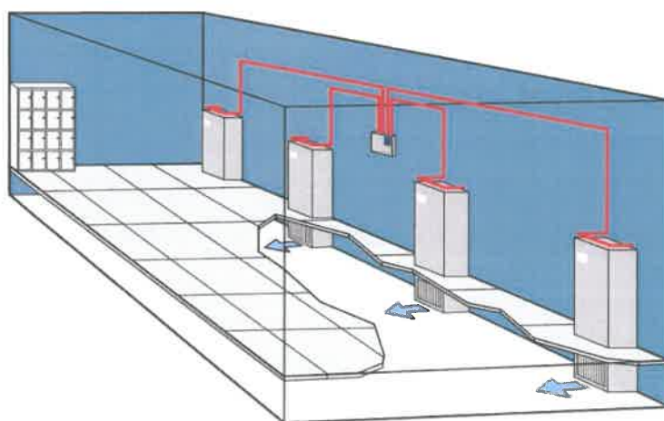
Primary Detection Example (All sampling points located directly in the airflow of the room at the return air grille of each handling unit)
